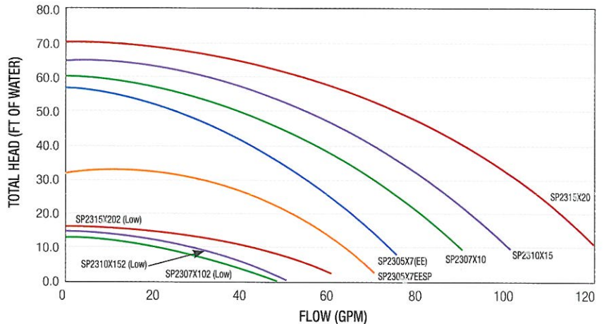
MAX-FLO XL FLOW VS TOTAL HEAD
